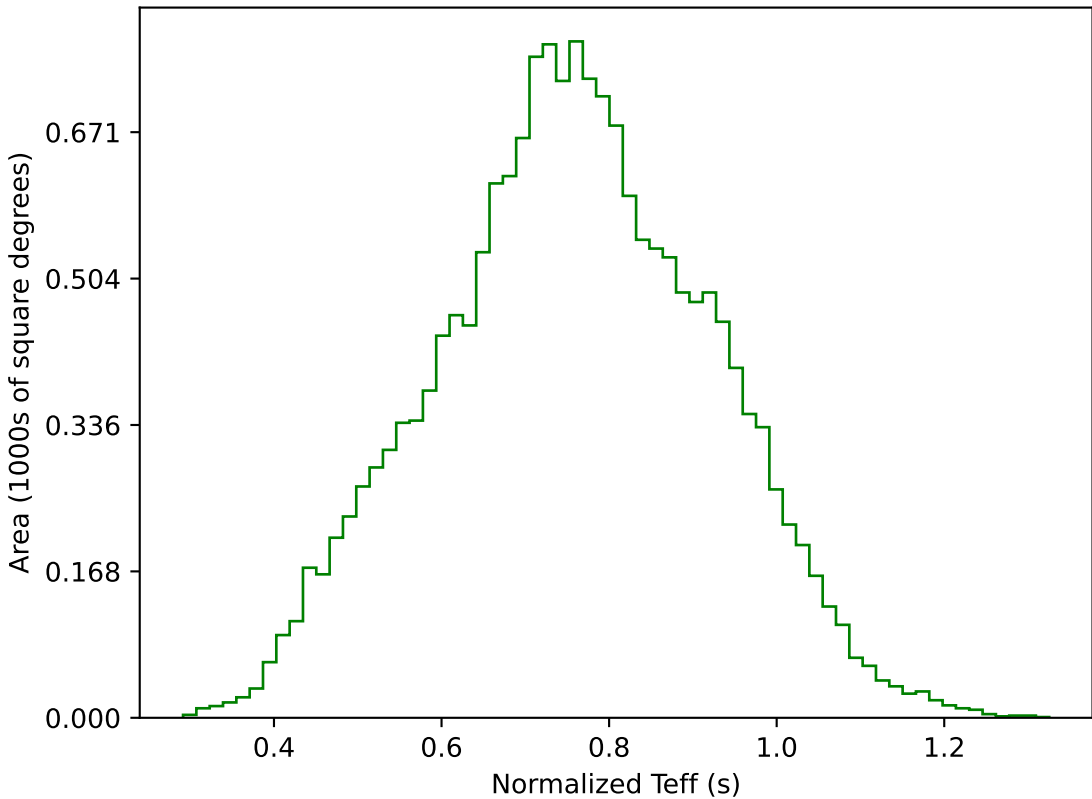
too_elab_r128_d2_gz_v3.4_10yrs WFD g band: Normalized Teff
