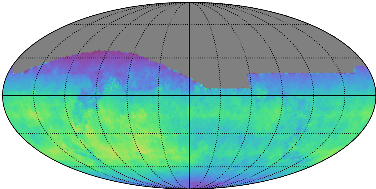
too_elab_r128_d2_gz_v3.4_10yrs All sky z band: Normalized Teff
