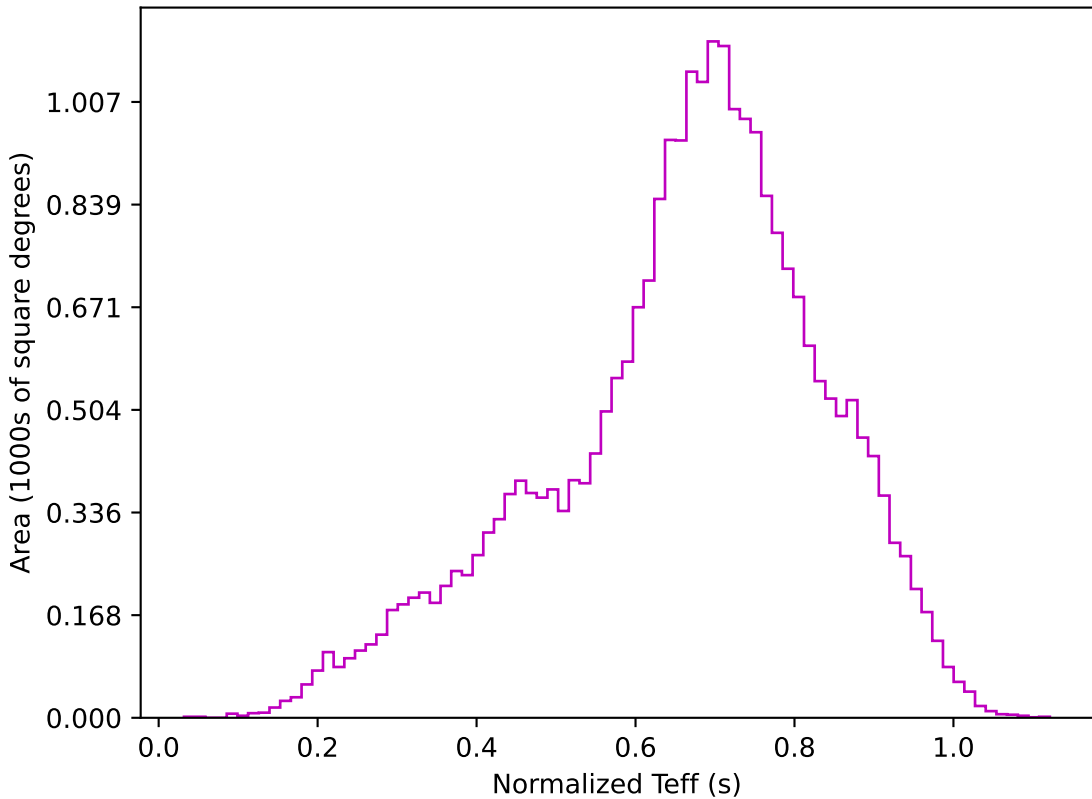
too_elab_r128_d2_gz_v3.4_10yrs All sky z band: Normalized Teff
