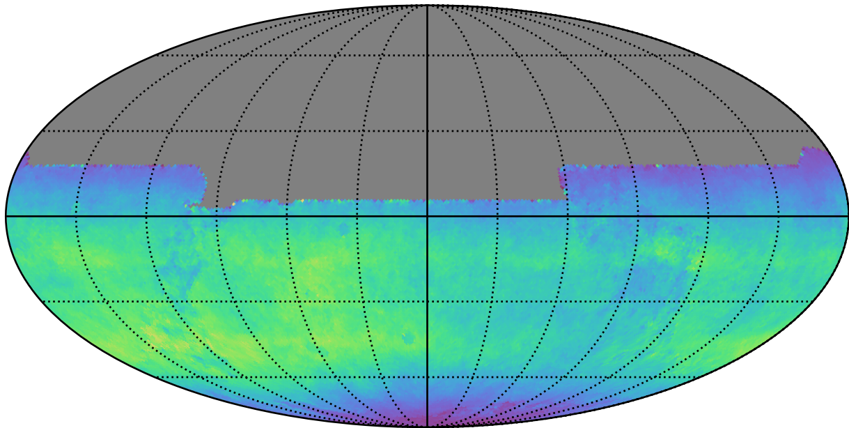
too_elab_r128_d2_gz_v3.4_10yrs All sky y band: Normalized Teff
