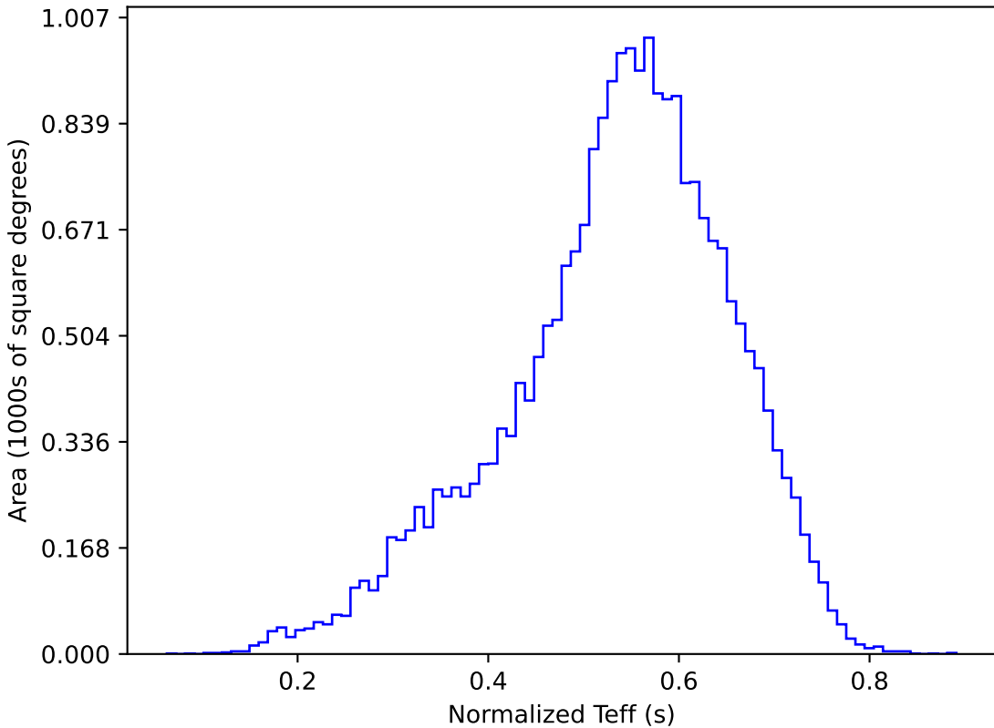
too_elab_r128_d2_gz_v3.4_10yrs All sky y band: Normalized Teff
