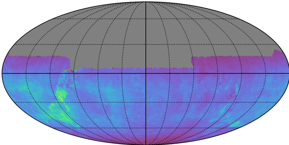
too_elab_r128_d2_gz_v3.4_10yrs All sky u band: Normalized Teff
