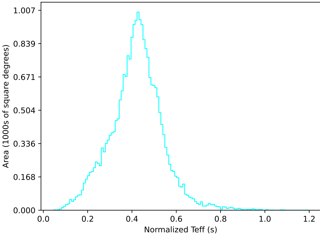
too_elab_r128_d2_gz_v3.4_10yrs All sky u band: Normalized Teff
