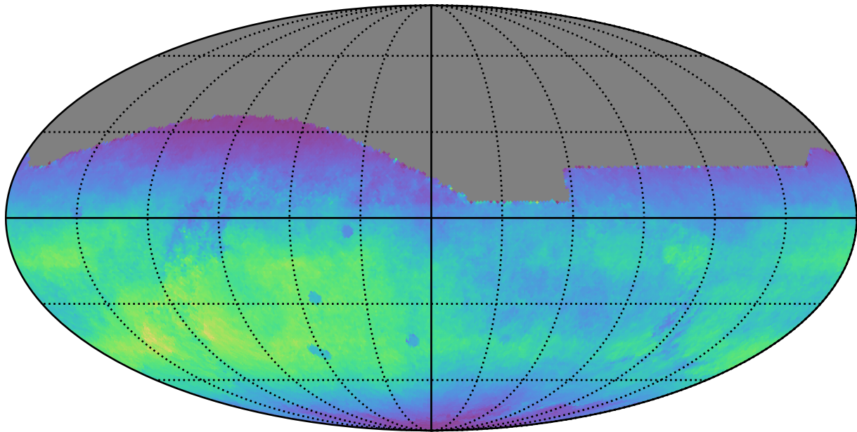
too_elab_r128_d2_gz_v3.4_10yrs All sky r band: Normalized Teff
