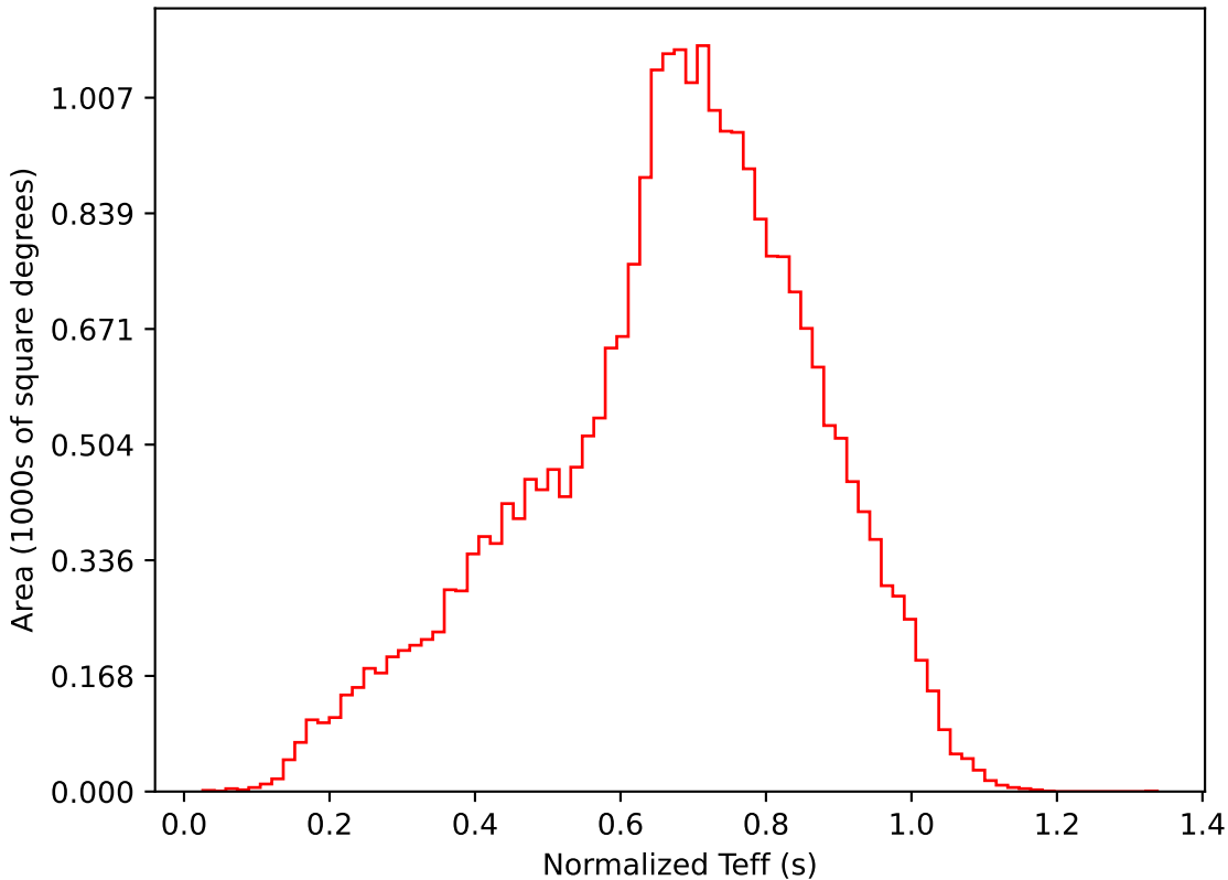
too_elab_r128_d2_gz_v3.4_10yrs All sky i band: Normalized Teff
