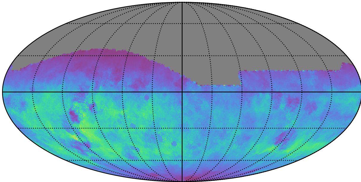
too_elab_r128_d2_gz_v3.4_10yrs All sky g band: Normalized Teff
