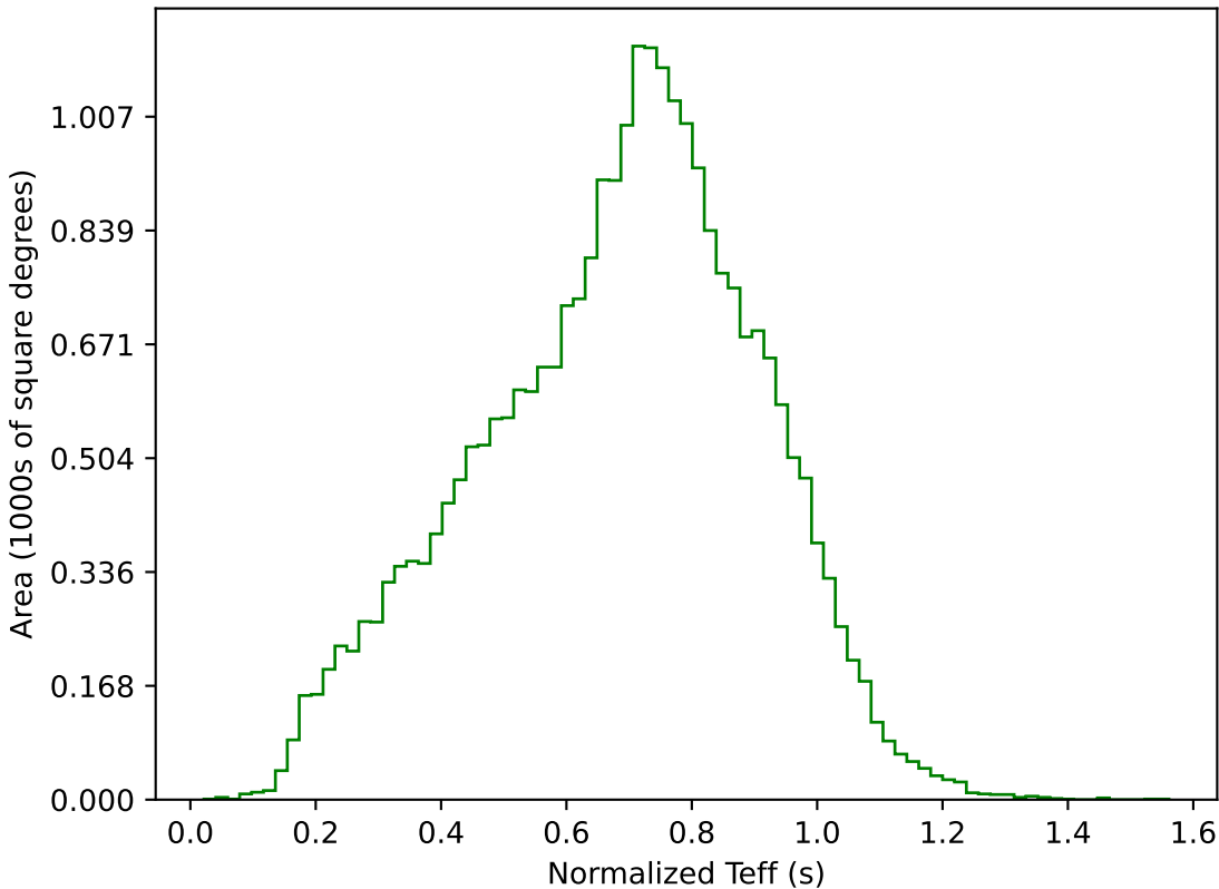
too_elab_r128_d2_gz_v3.4_10yrs All sky g band: Normalized Teff
