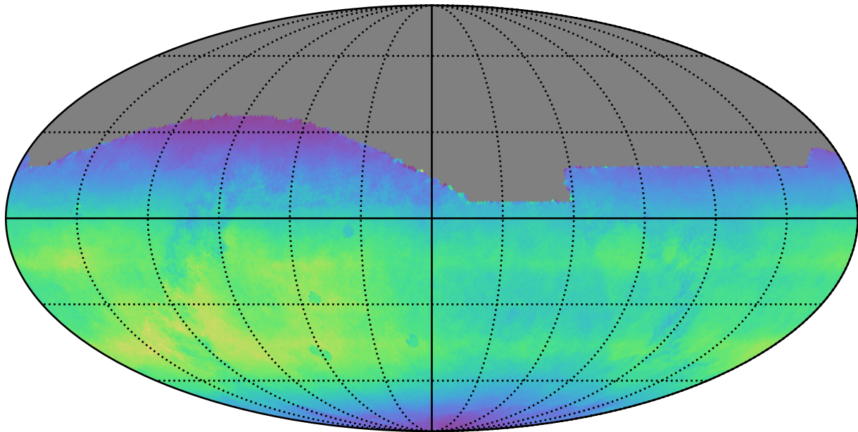
too_elab_r128_d2_gz_v3.4_10yrs All sky all bands: Normalized Teff
