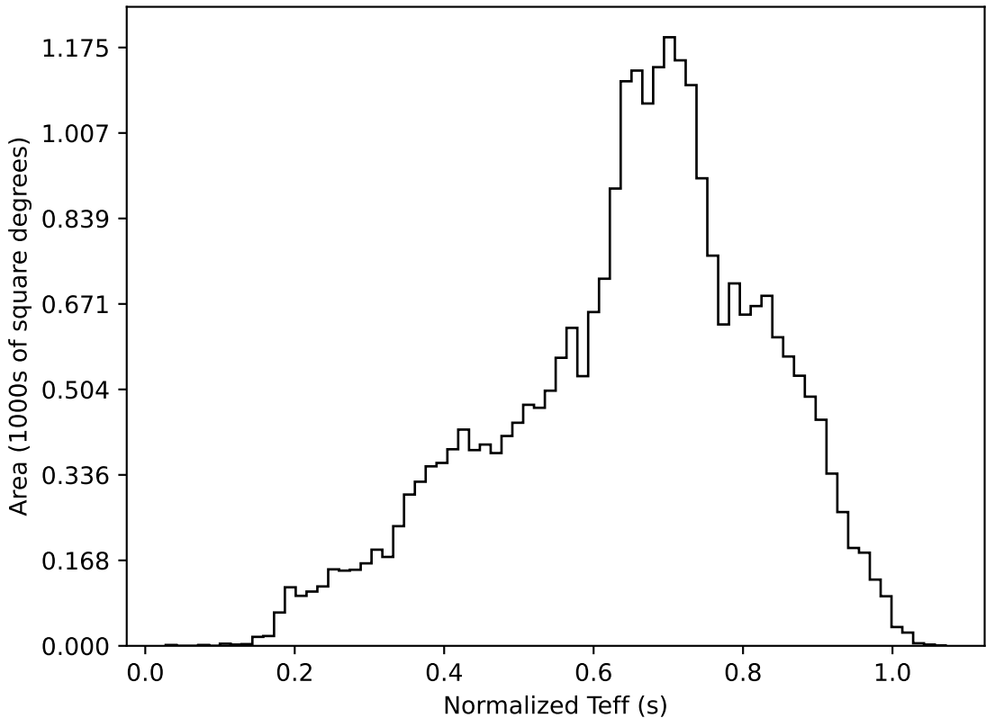
too_elab_r128_d2_gz_v3.4_10yrs All sky all bands: Normalized Teff
