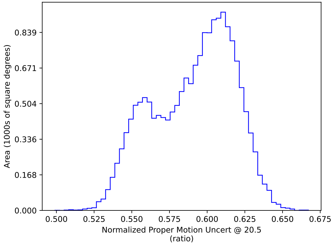
too_elab_r128_d2_gz_v3.4_10yrs WFD: Normalized Proper Motion Uncert @ 20.5
