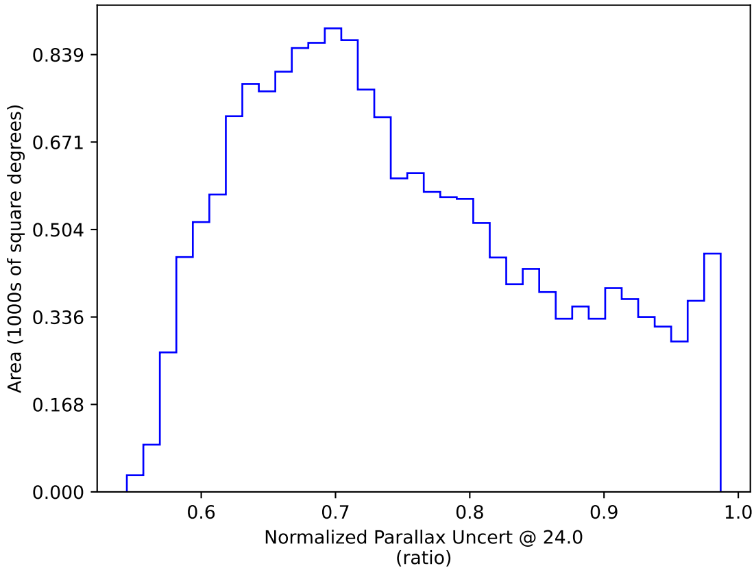
too_elab_r128_d2_gz_v3.4_10yrs WFD: Normalized Parallax Uncert @ 24.0
