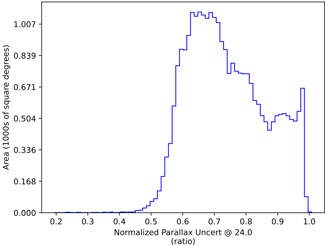
too_elab_r128_d2_gz_v3.4_10yrs All sky: Normalized Parallax Uncert @ 24.0
