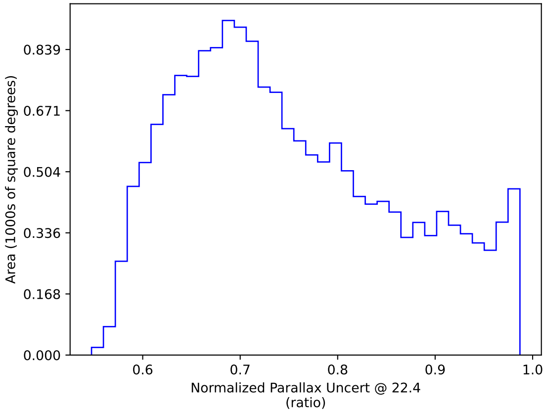
too_elab_r128_d2_gz_v3.4_10yrs WFD: Normalized Parallax Uncert @ 22.4
