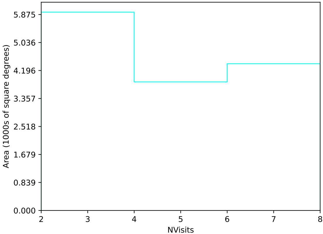
too_elab_r128_d2_gz_v3.4_10yrs Yr 3-4 u band: NVisits
