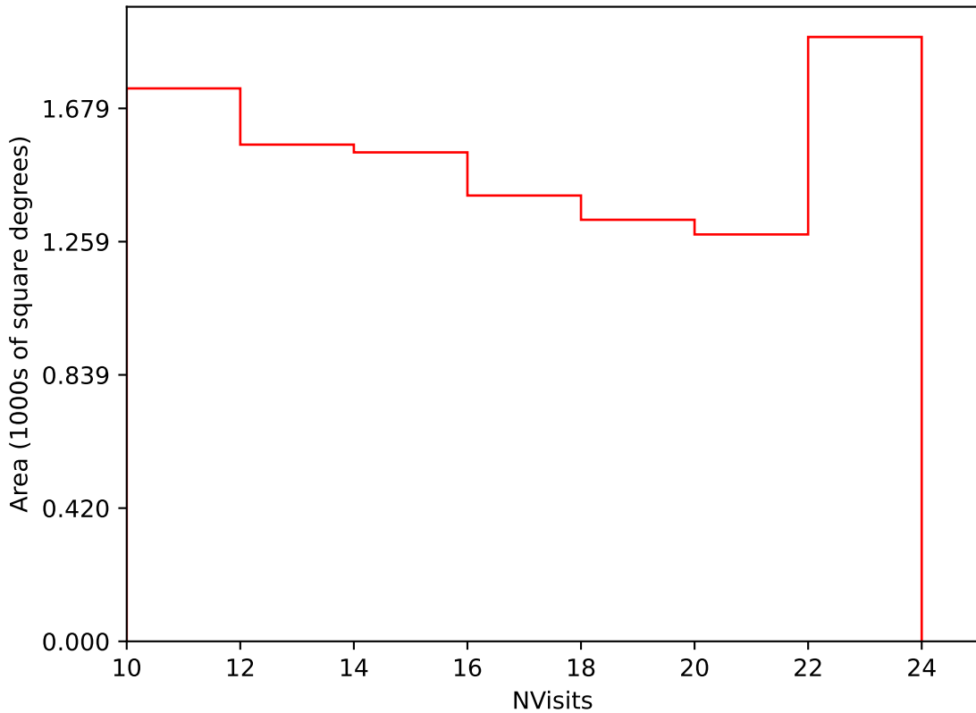
too_elab_r128_d2_gz_v3.4_10yrs Yr 3-4 i band: NVisits
