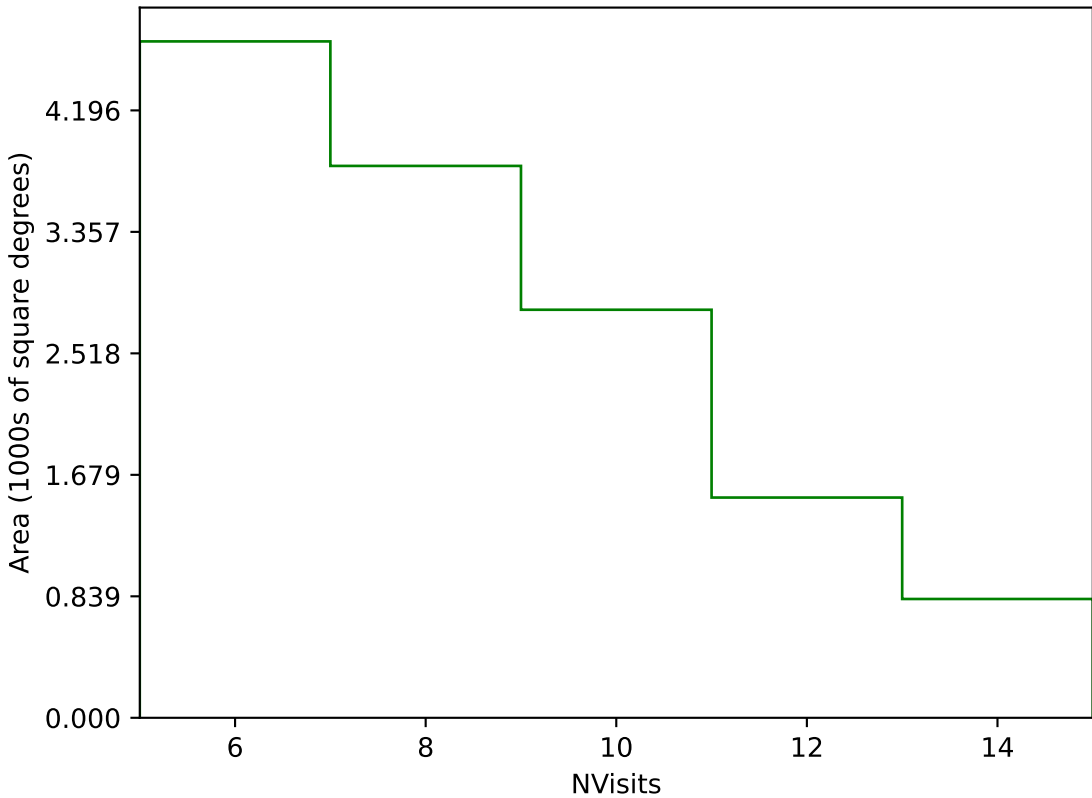
too_elab_r128_d2_gz_v3.4_10yrs Yr 3-4 g band: NVisits
