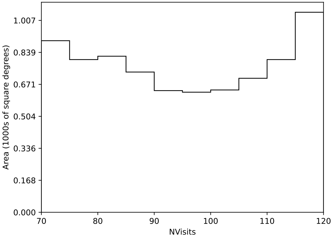
too_elab_r128_d2_gz_v3.4_10yrs Yr 3-4 all bands: NVisits
