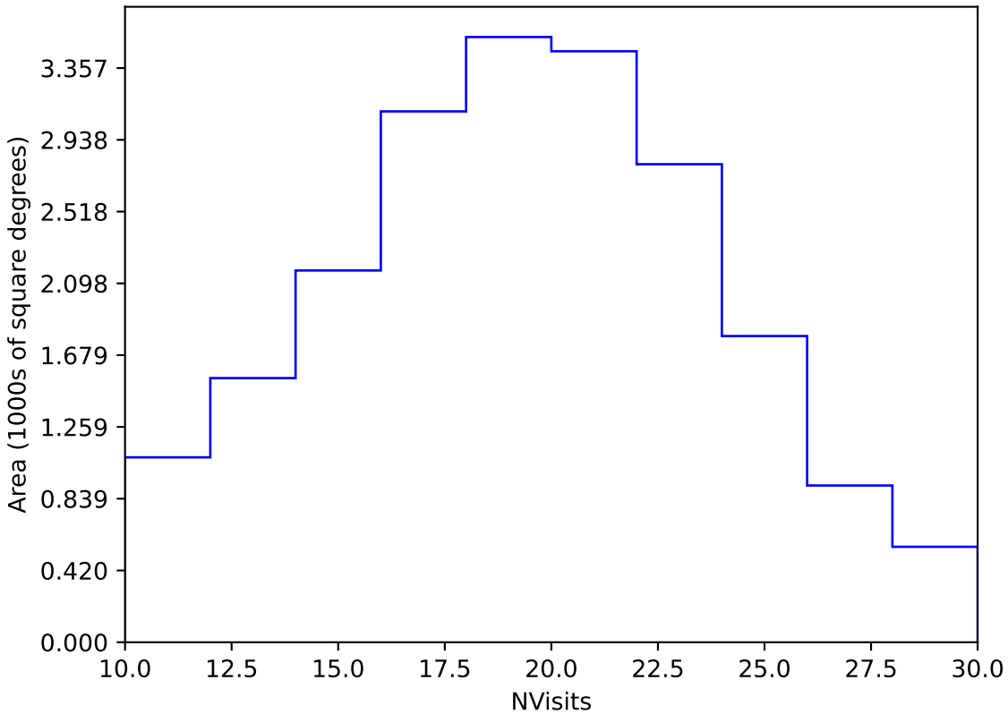
too_elab_r128_d2_gz_v3.4_10yrs Yr 1 y band: NVisits
