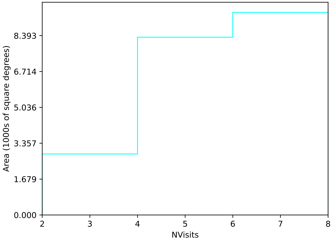
too_elab_r128_d2_gz_v3.4_10yrs Yr 1 u band: NVisits
