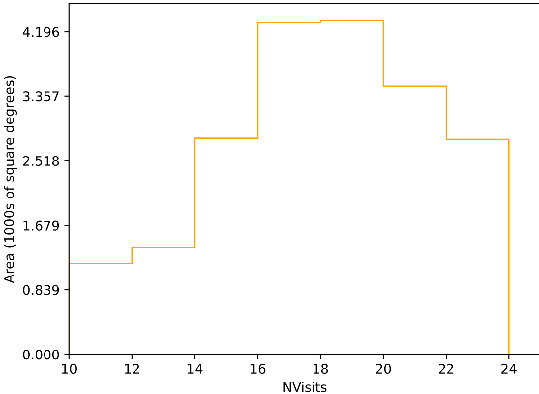
too_elab_r128_d2_gz_v3.4_10yrs Yr 1 r band: NVisits
