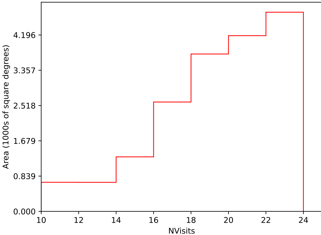
too_elab_r128_d2_gz_v3.4_10yrs Yr 1 i band: NVisits
