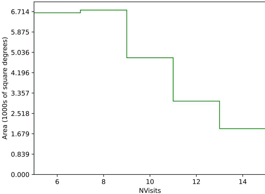
too_elab_r128_d2_gz_v3.4_10yrs Yr 1 g band: NVisits
