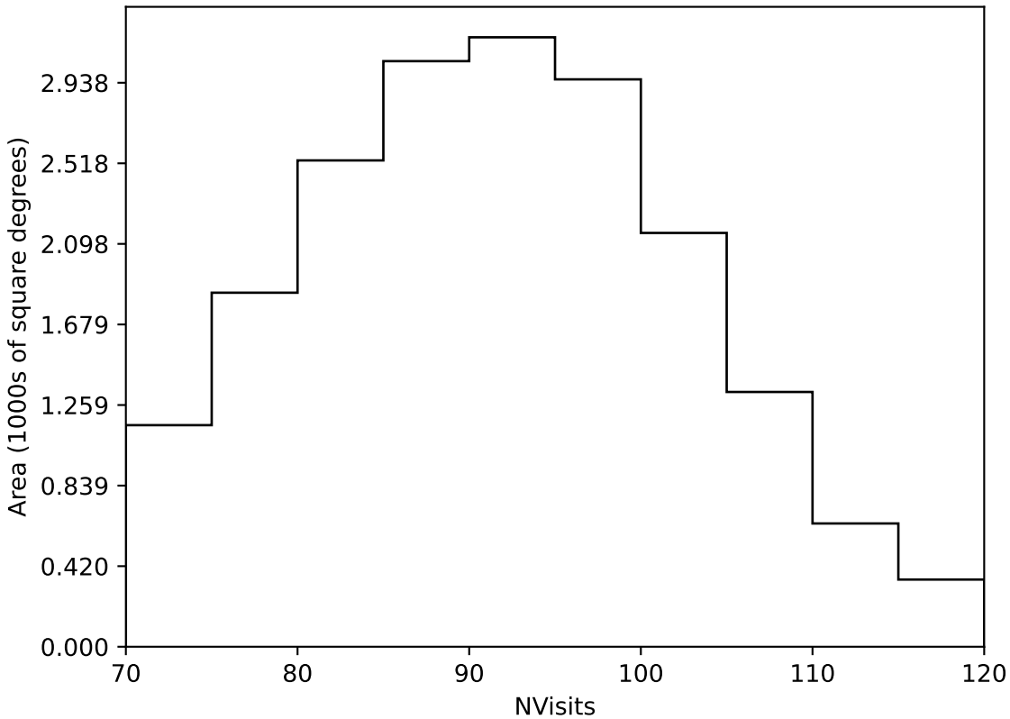
too_elab_r128_d2_gz_v3.4_10yrs Yr 1 all bands: NVisits
