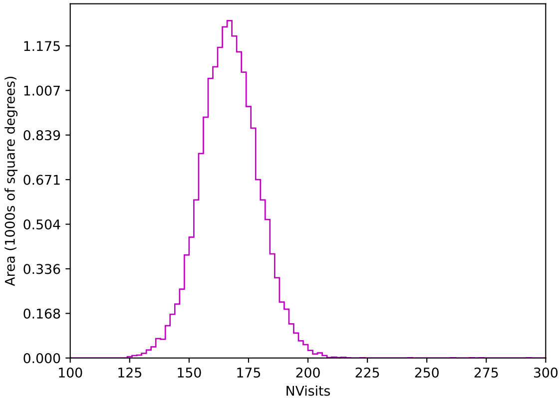
too_elab_r128_d2_gz_v3.4_10yrs WFD z band: NVisits
