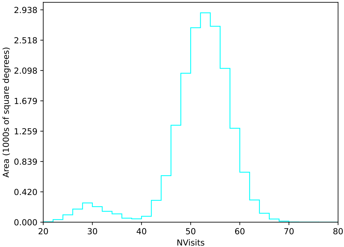
too_elab_r128_d2_gz_v3.4_10yrs WFD u band: NVisits
