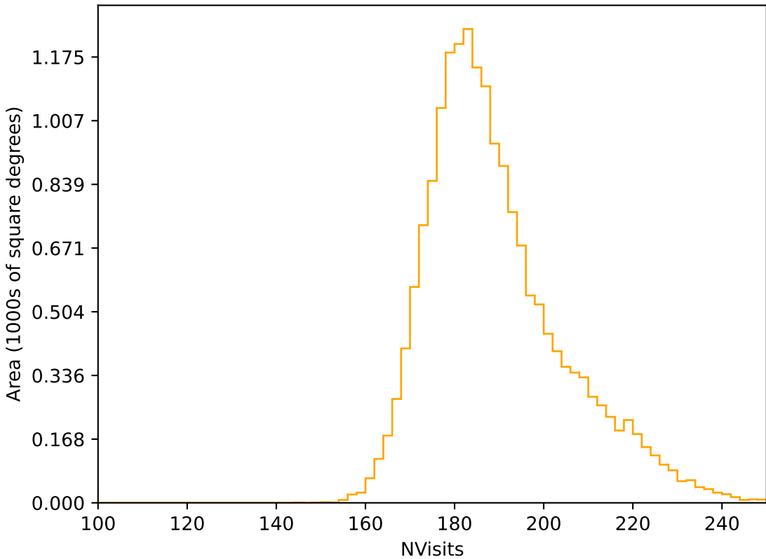
too_elab_r128_d2_gz_v3.4_10yrs WFD r band: NVisits
