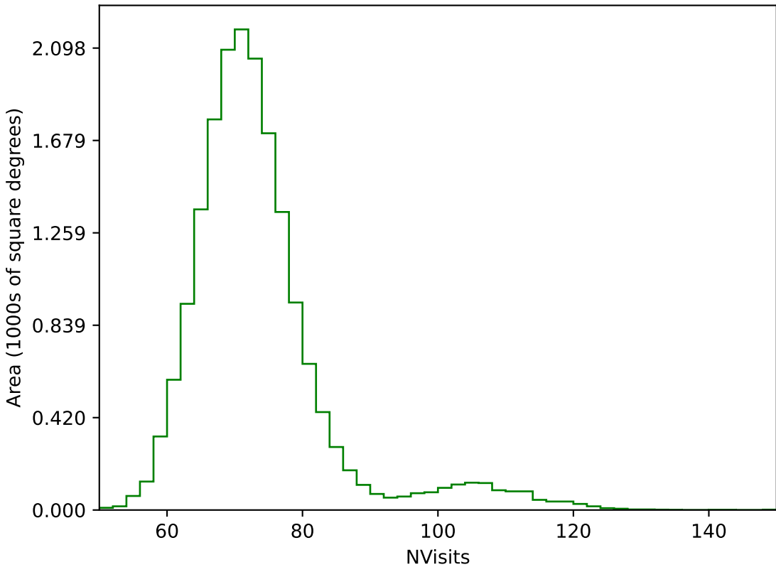
too_elab_r128_d2_gz_v3.4_10yrs WFD g band: NVisits
