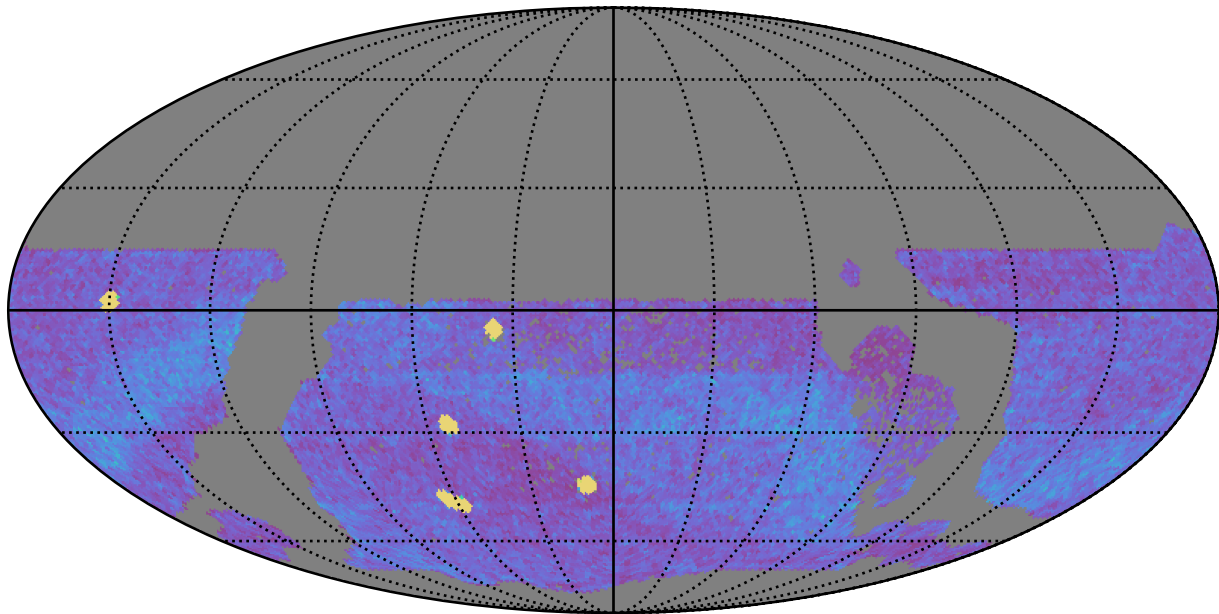
too_elab_r128_d2_gz_v3.4_10yrs WFD all bands: NVisits
