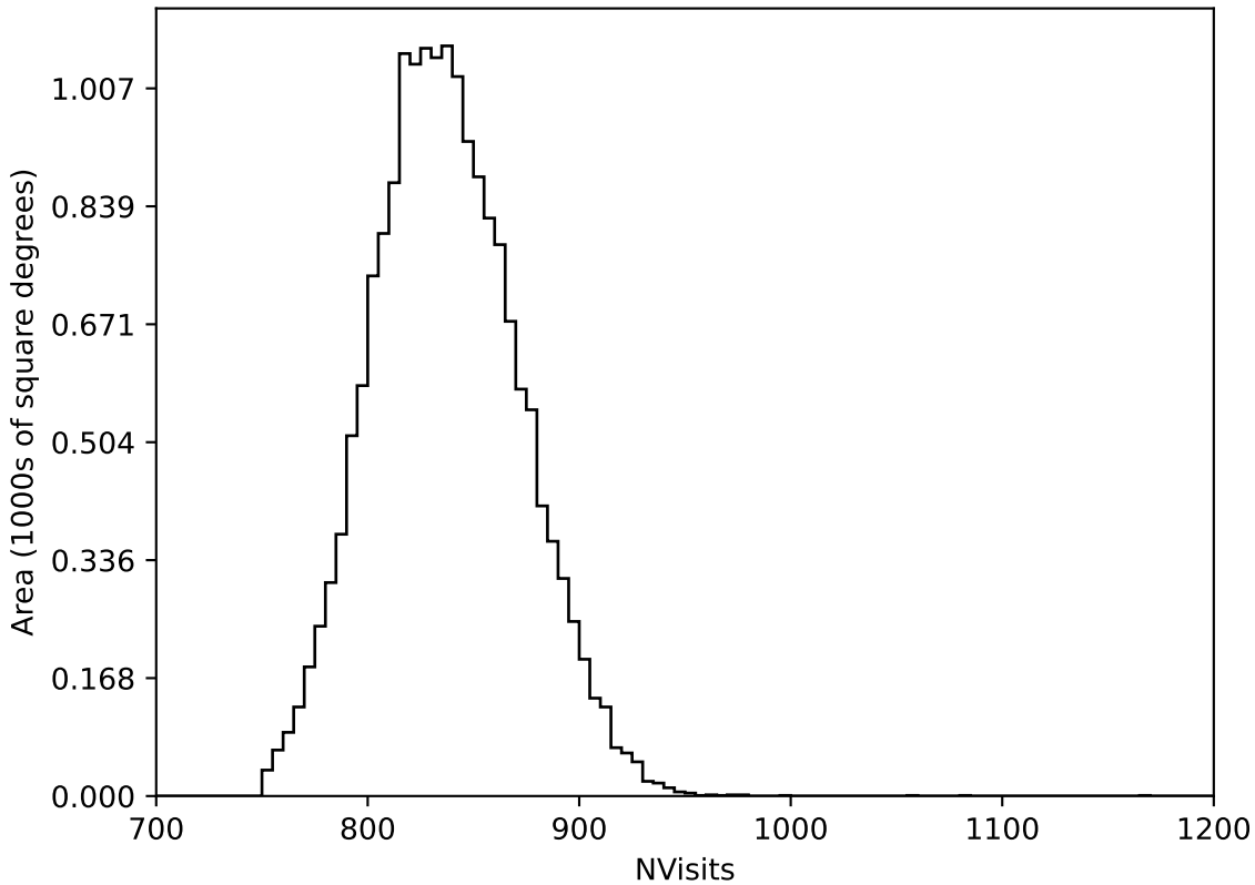
too_elab_r128_d2_gz_v3.4_10yrs WFD all bands: NVisits
