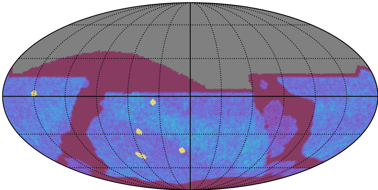
too_elab_r128_d2_gz_v3.4_10yrs All sky z band: NVisits
