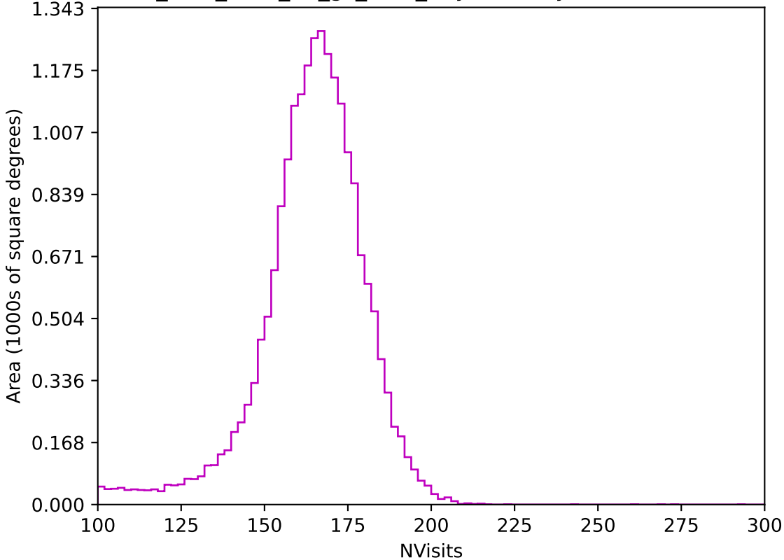
too_elab_r128_d2_gz_v3.4_10yrs All sky z band: NVisits
