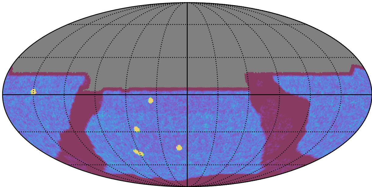
too_elab_r128_d2_gz_v3.4_10yrs All sky y band: NVisits
