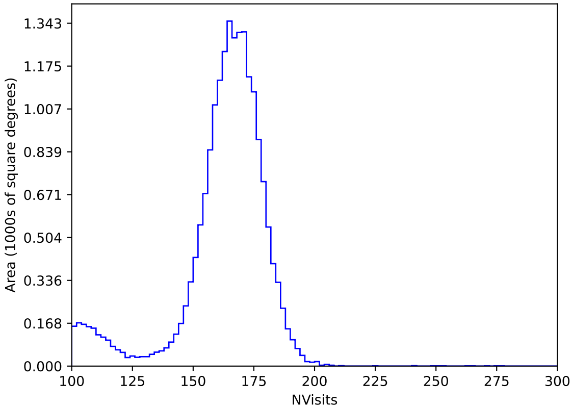
too_elab_r128_d2_gz_v3.4_10yrs All sky y band: NVisits
