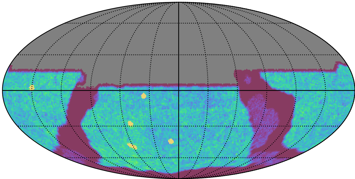
too_elab_r128_d2_gz_v3.4_10yrs All sky u band: NVisits
