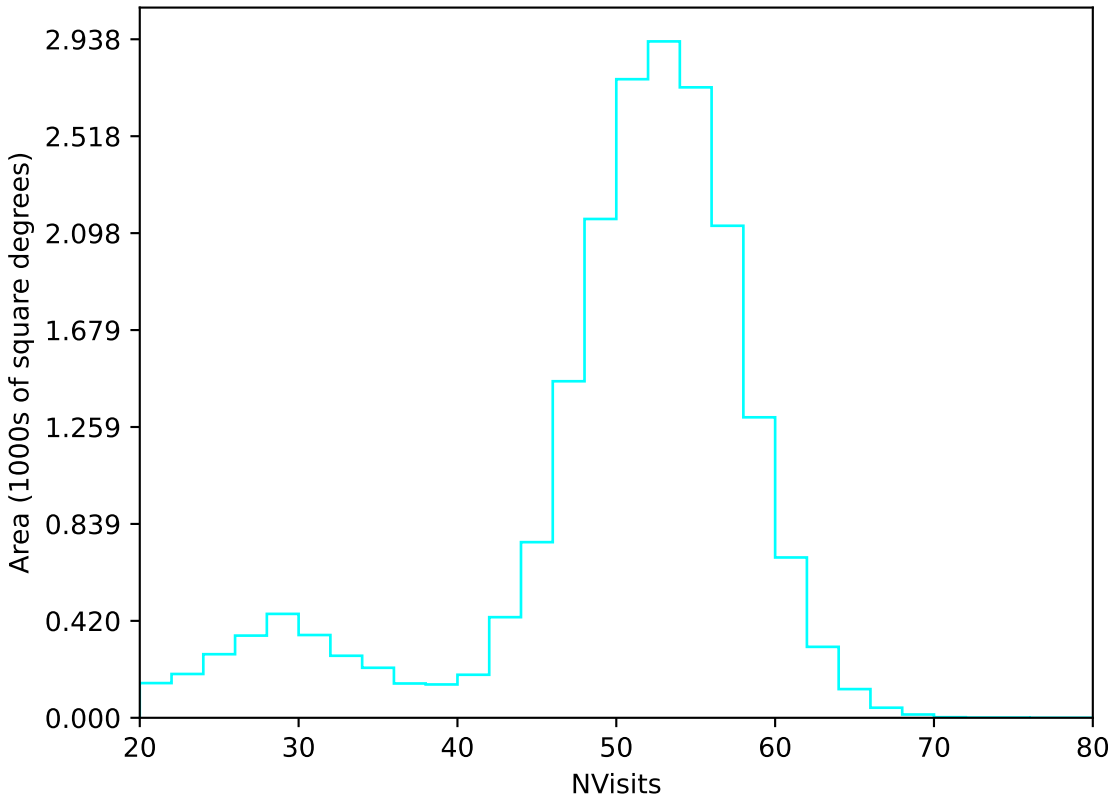
too_elab_r128_d2_gz_v3.4_10yrs All sky u band: NVisits
