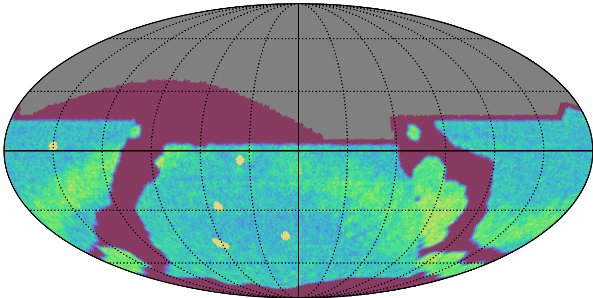
too_elab_r128_d2_gz_v3.4_10yrs All sky r band: NVisits
