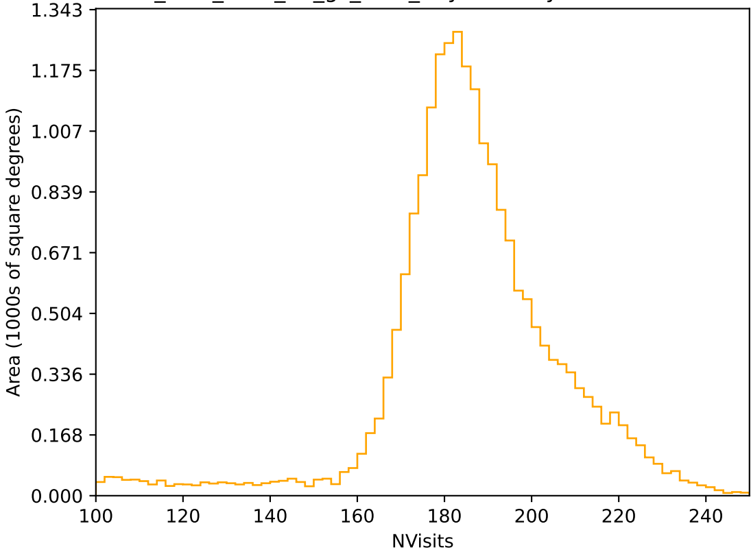
too_elab_r128_d2_gz_v3.4_10yrs All sky r band: NVisits
