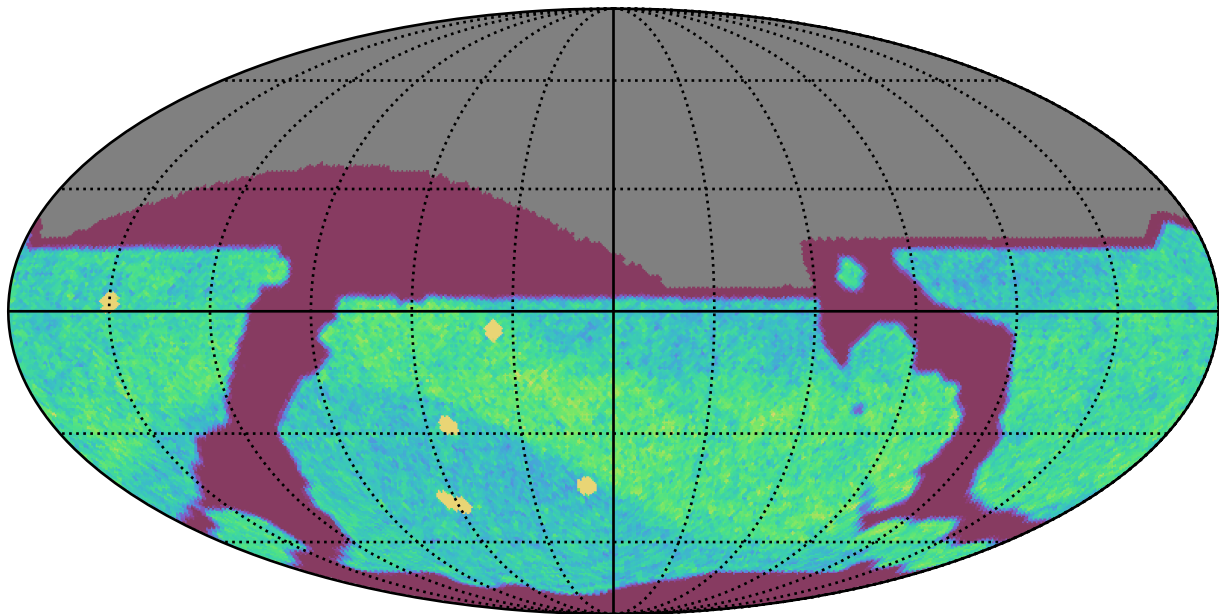
too_elab_r128_d2_gz_v3.4_10yrs All sky i band: NVisits
