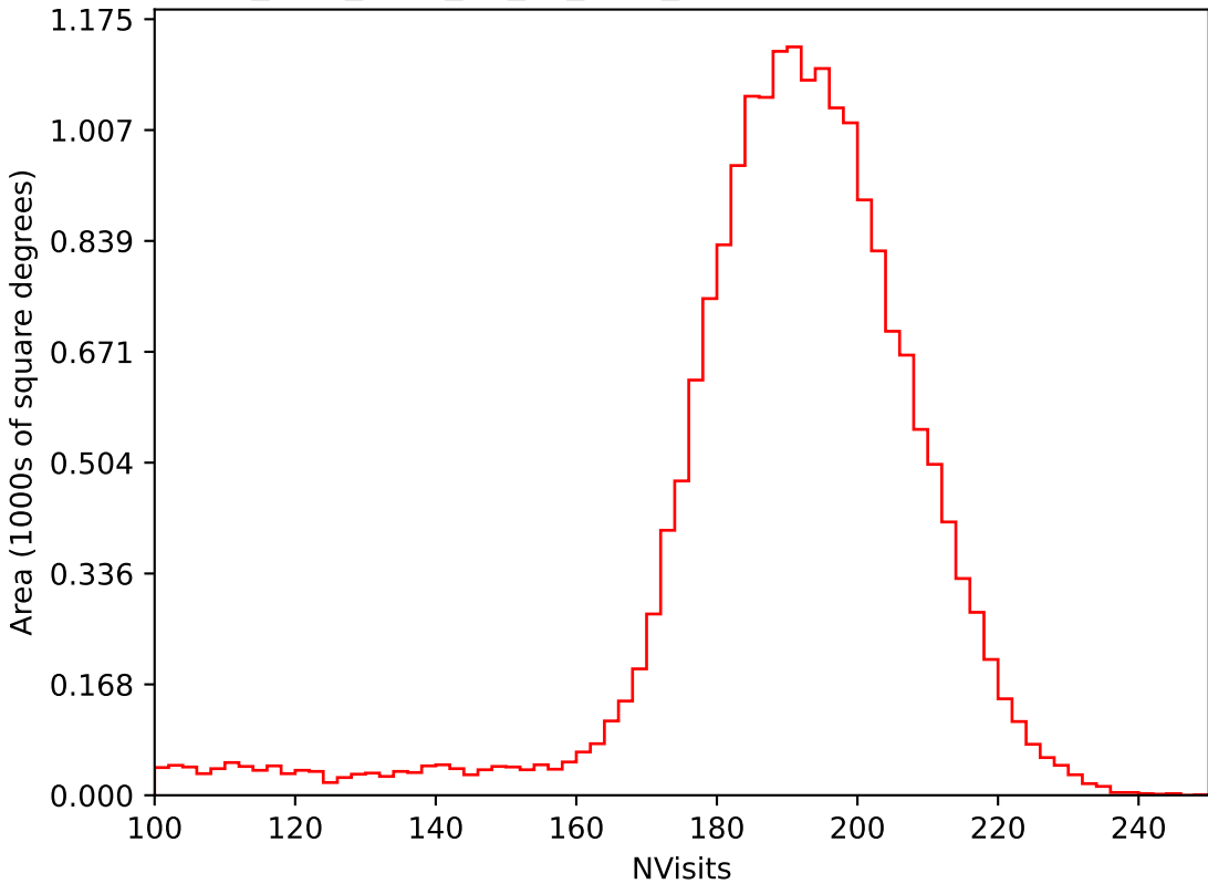
too_elab_r128_d2_gz_v3.4_10yrs All sky i band: NVisits
