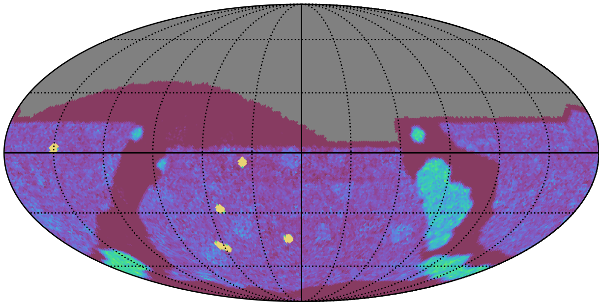
too_elab_r128_d2_gz_v3.4_10yrs All sky g band: NVisits
