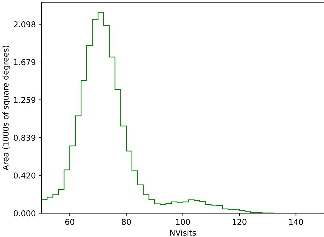
too_elab_r128_d2_gz_v3.4_10yrs All sky g band: NVisits
