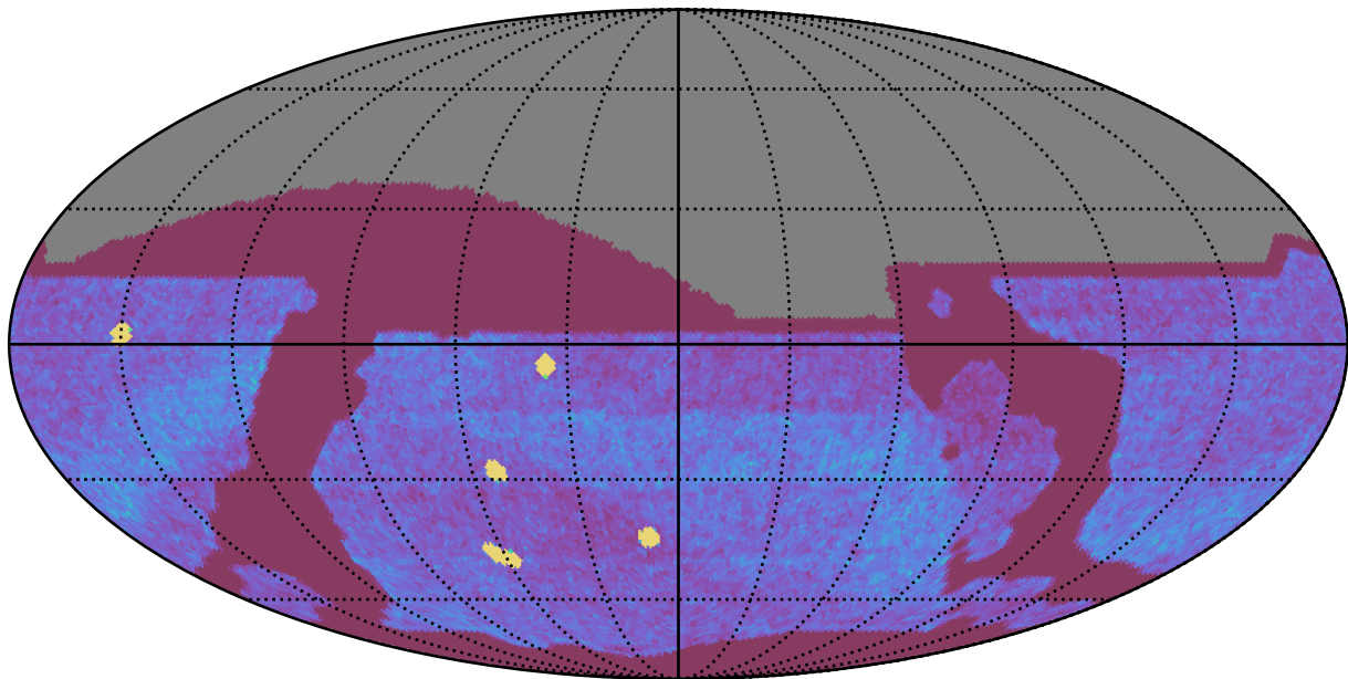
too_elab_r128_d2_gz_v3.4_10yrs All sky all bands: NVisits
