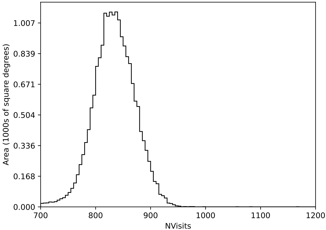
too_elab_r128_d2_gz_v3.4_10yrs All sky all bands: NVisits
