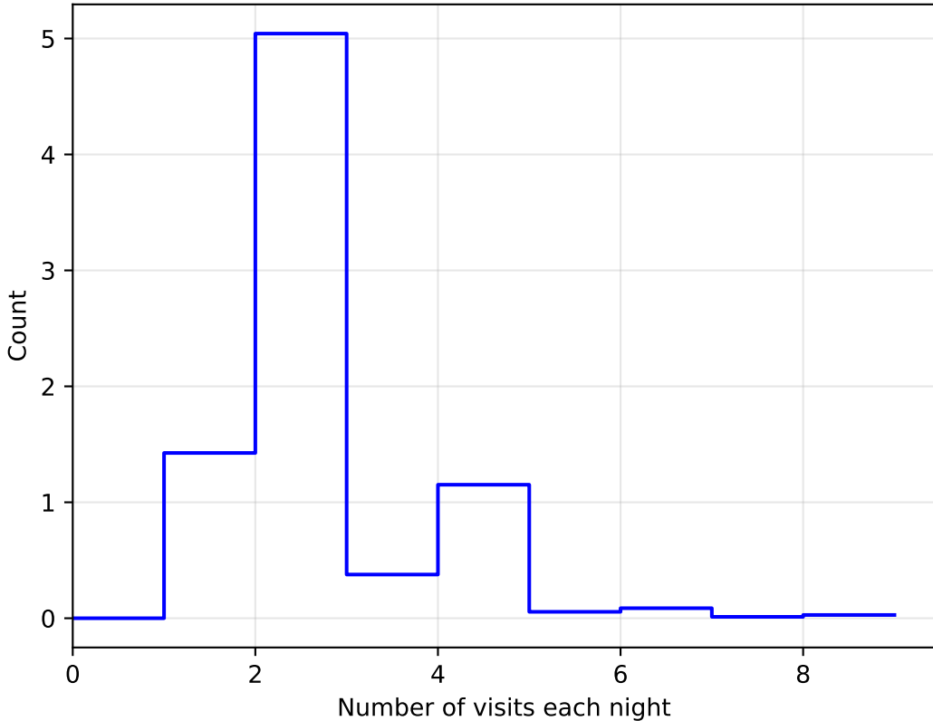
too_elab_r128_d2_gz_v3.4_10yrs WFD: NVisitsPerNight
