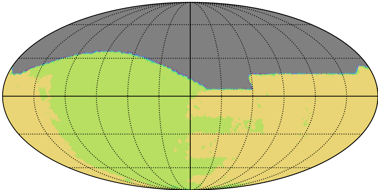
too_elab_r128_d2_gz_v3.4_10yrs All sky all bands: NSeasons
