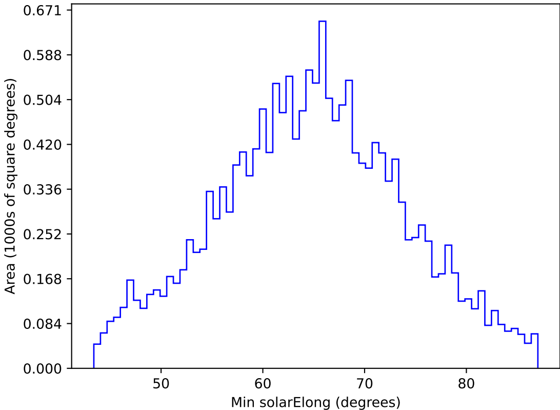
too_elab_r128_d2_gz_v3.4_10yrs WFD y band: Min solarElong
